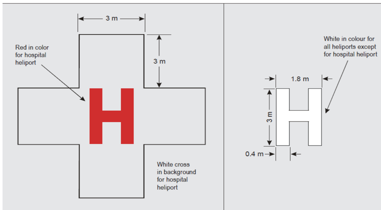
Figure 5-3. Hospital heliport identification and heliport identification marking
