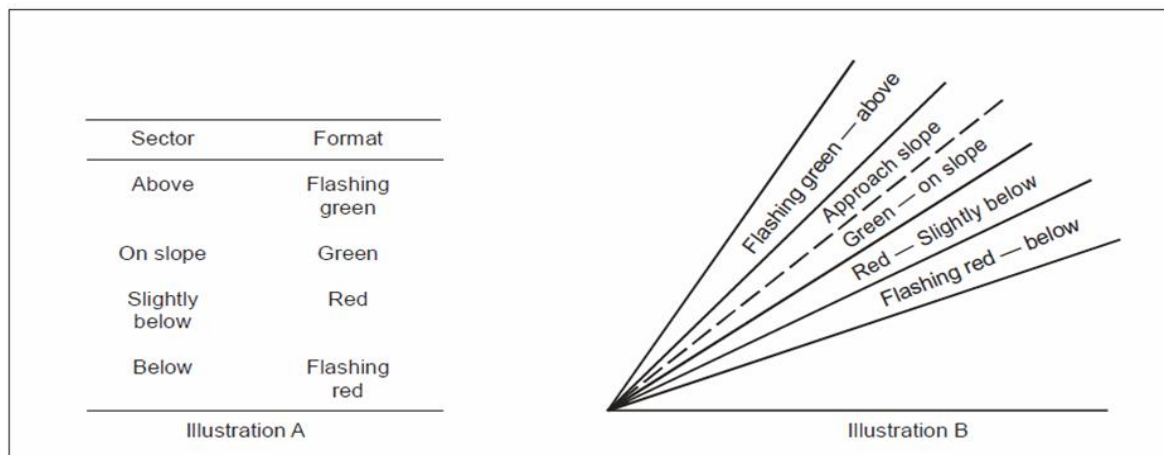
Figure 5-15. HAPI signal format
