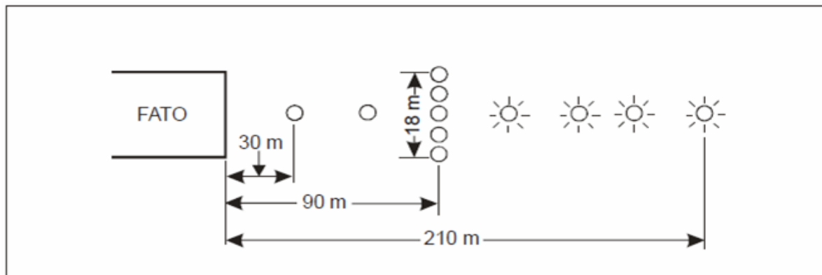
Figure 5-12. Approach lighting system
