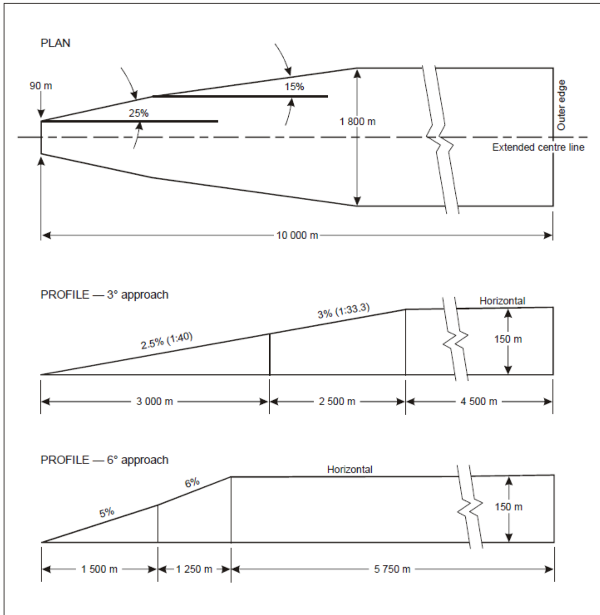
Figure A1-3. Approach surface for precision approach FATO
