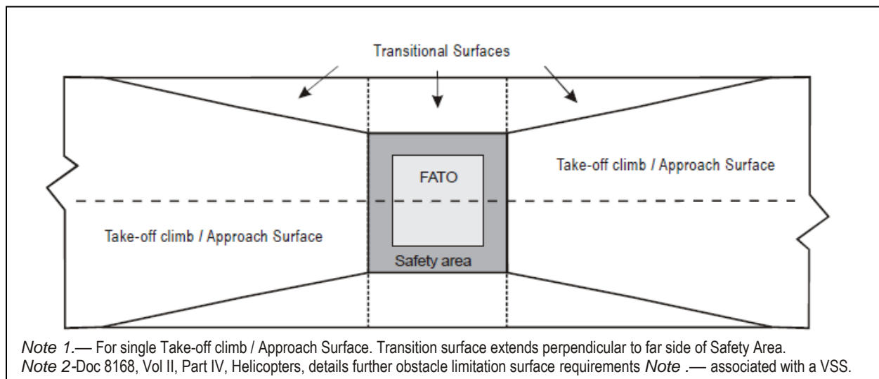
Figure A1-4. Approach surface for non-precision approach FATO
