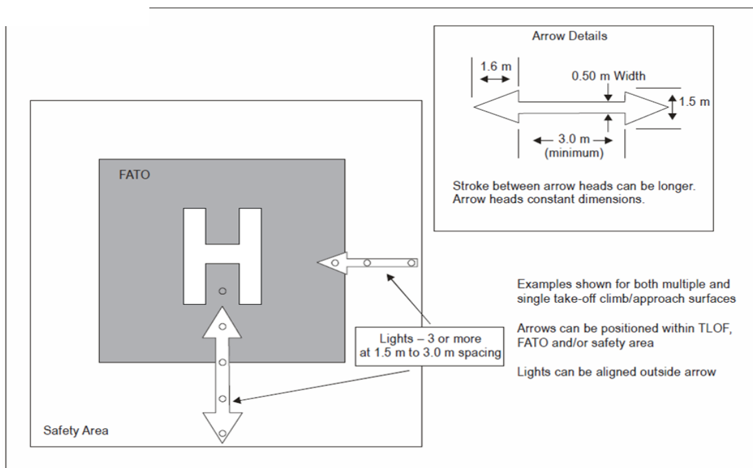
Figure 5-9. Flight path alignment guidance markings and lights
