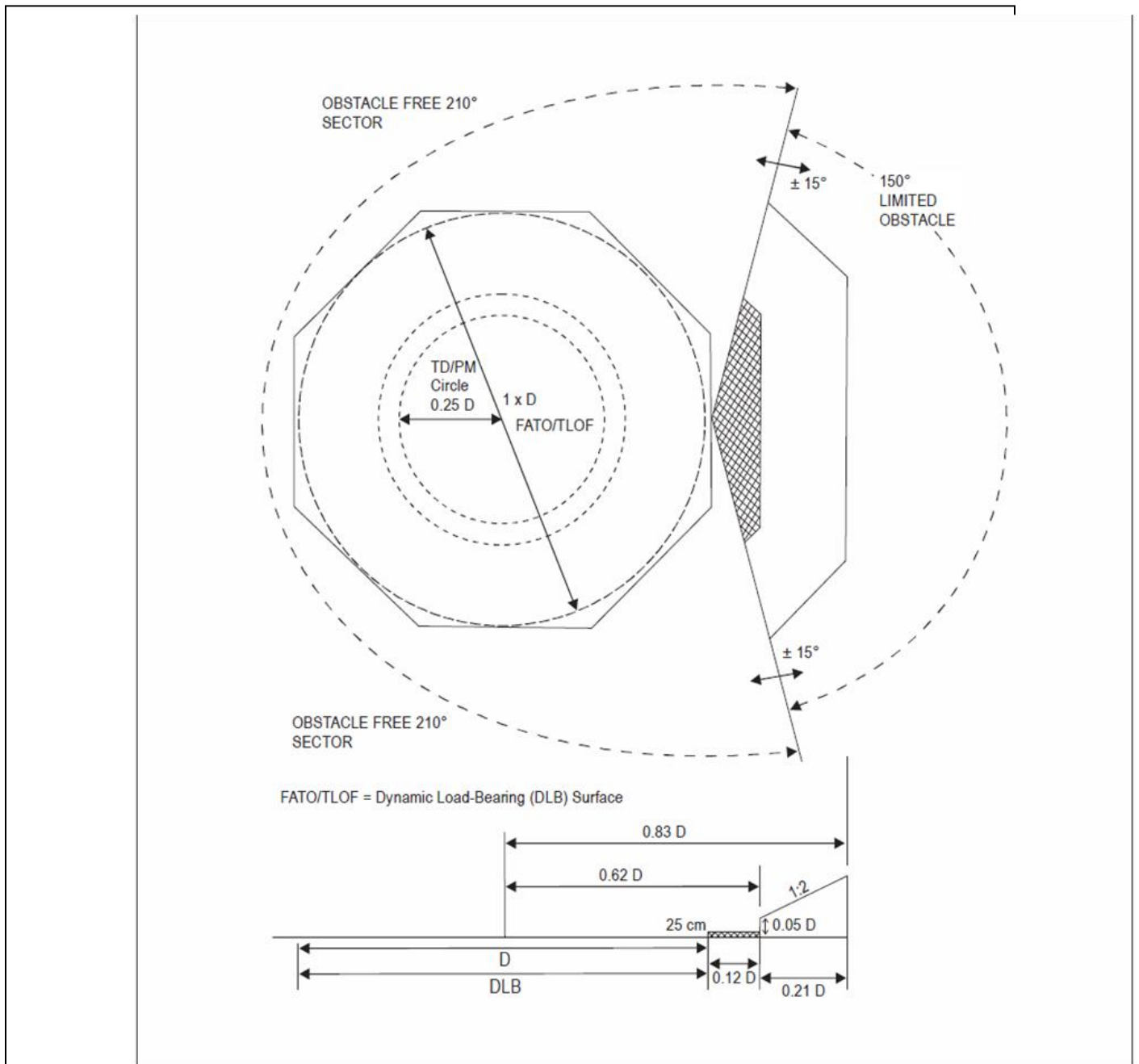
Figure 4-8. Helideck obstacle limitation sectors and surfaces for a FATO and coincidental TLOF of 1 D and larger
