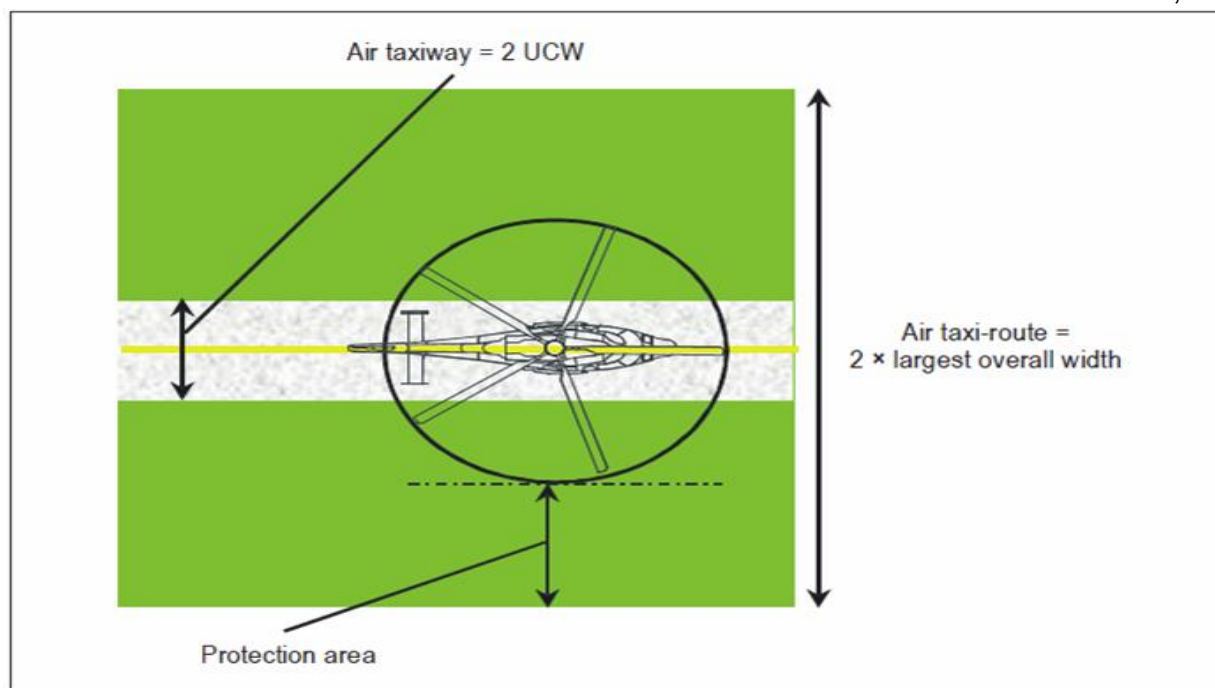
Figure 3-3. Helicopter air taxi-route/taxiway
