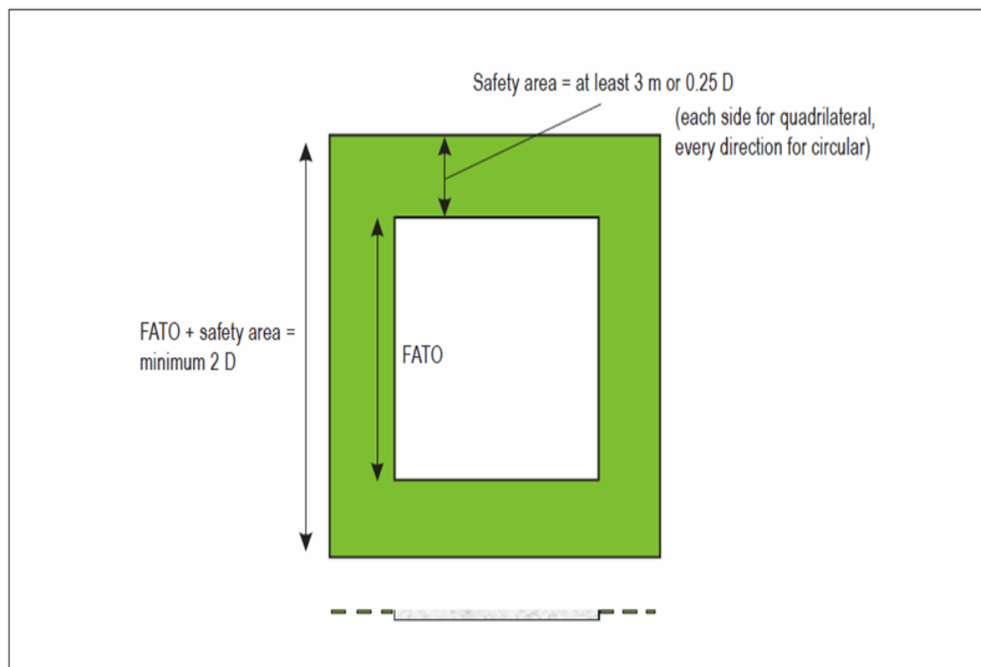
Figure 3-1. FATO and associated safety area
