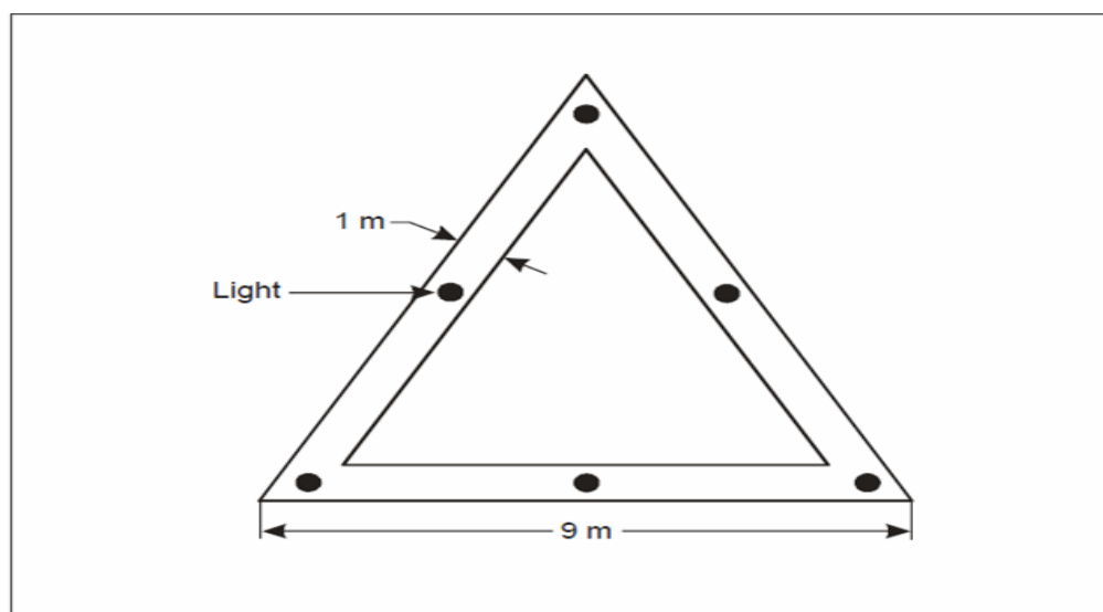
Figure 5-6. Aiming point marking
