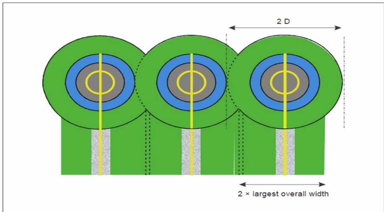
Figure 3-5. Helicopter stands designed for hover turns with air taxi-routes/taxiways — simultaneous operations
