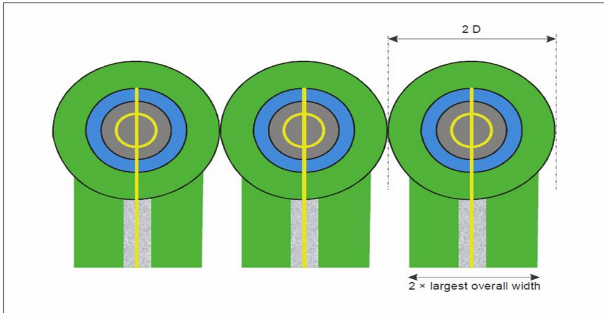
Figure 3-5. Helicopter stands designed for hover turns with air taxi-routes/taxiways — simultaneous operations
