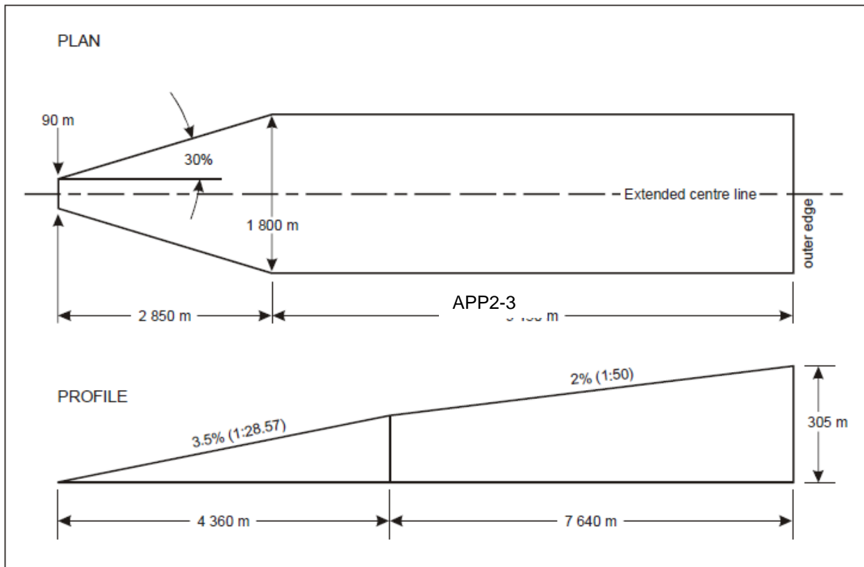
Figure A1-2 Take-off climb surface for instrument FATO
