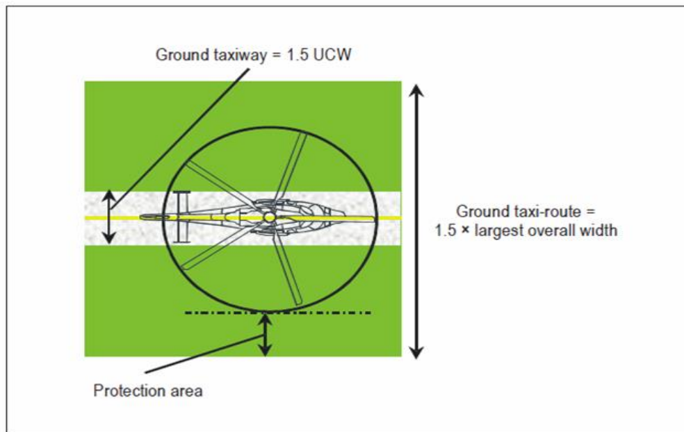
Figure 3-2. Helicopter ground taxi-route/taxiway
