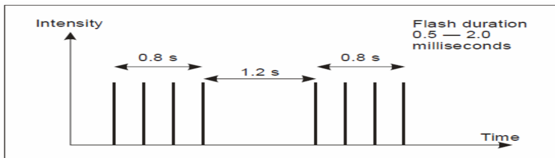
Figure 5-10. Heliport beacon flash characteristics
