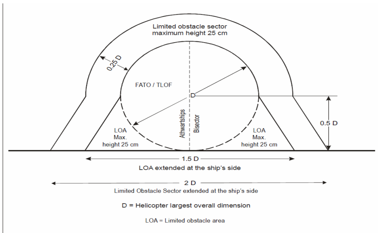
Figure 4-11. Ships-side non-purpose-built heliport obstacle limitation sectors and surfaces
