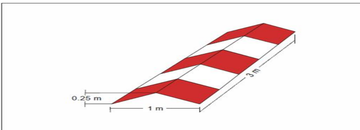
Figure 5-5. Runway-type FATO edge marker
