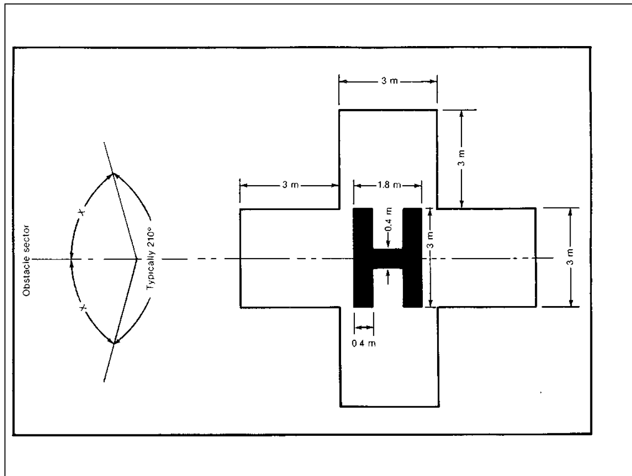
Figure 5-1. Helipoint identification marking
