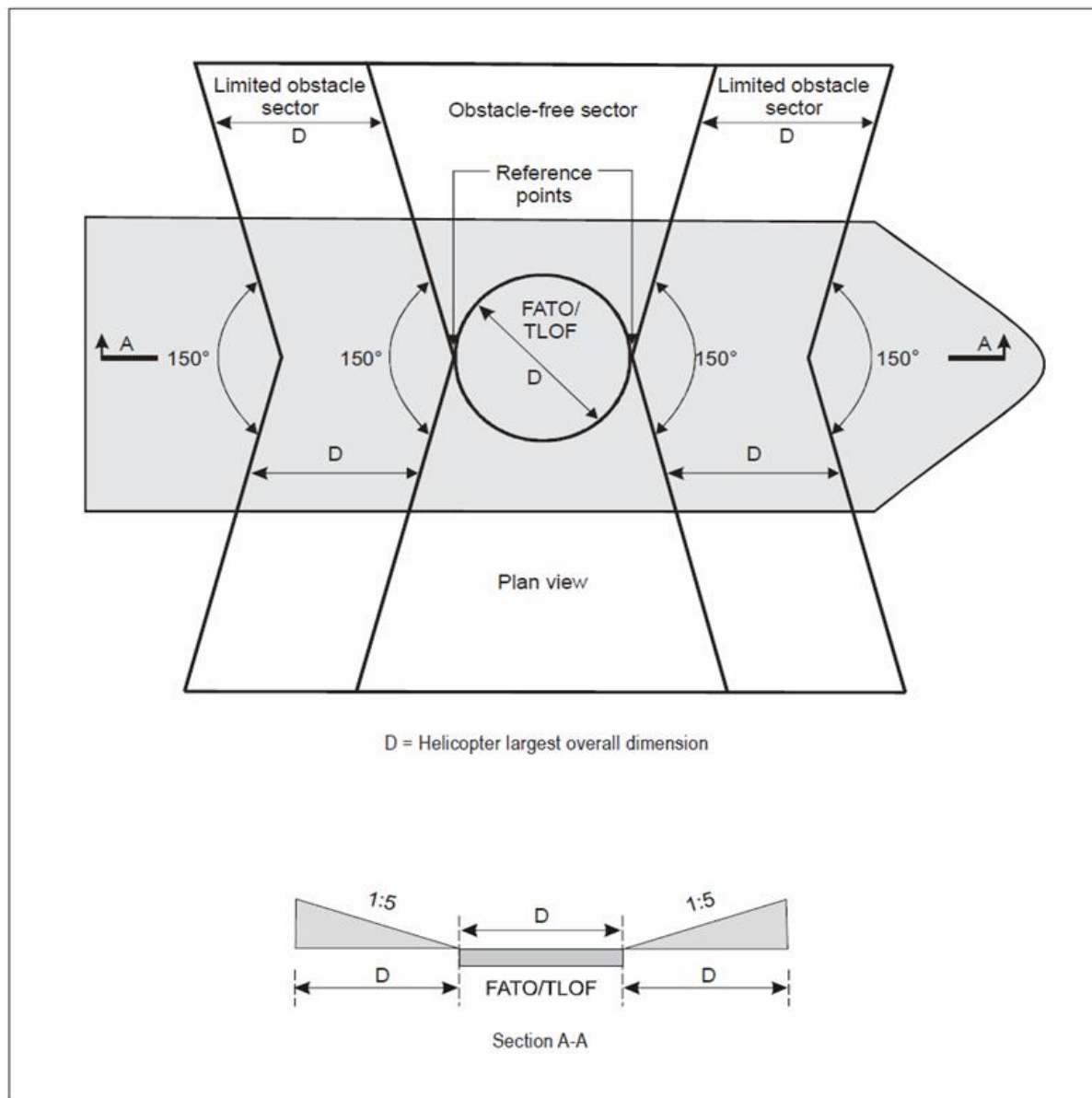
Figure 4-10. Amidship's location — Shipboard heliport obstacle limitation surfaces
