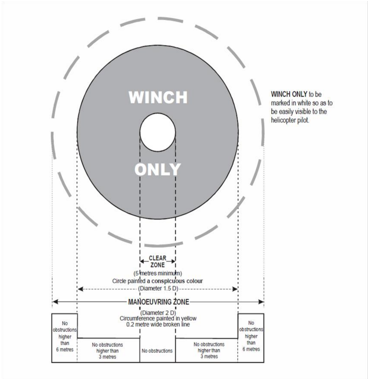
Figure 4-12. Winching area of a ship
