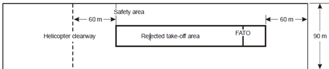
Figure A1-1 safety area for instrument FATO
